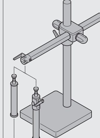
Stand A consisting of: - Boom A 000000-1046-522 - Stand base 10/260x260 000000-1046-518
