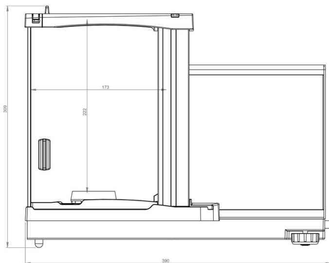
XA 21.5Y.M Microbalance
