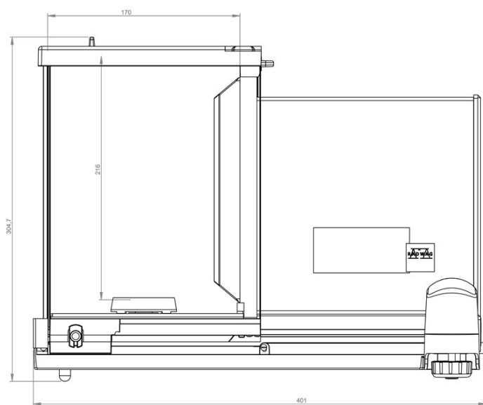
XA 21.5Y.M.A Microbalance
