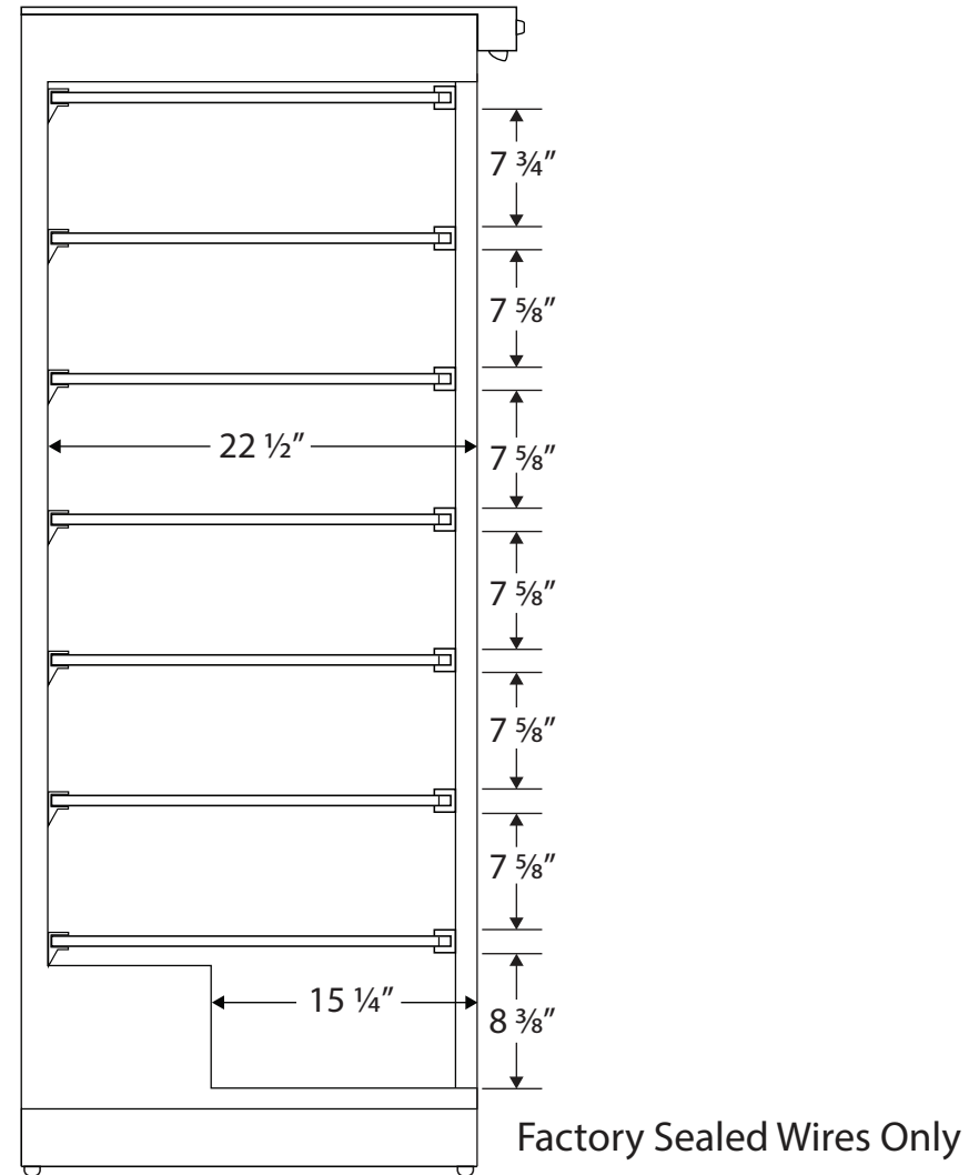
Side View
