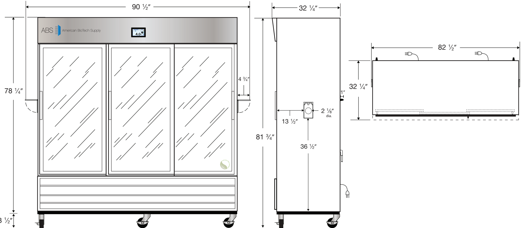
Top View
