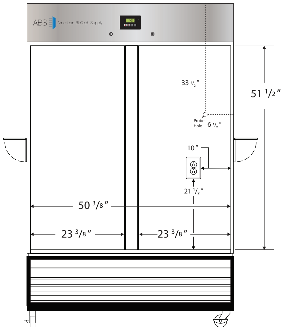
Front View
