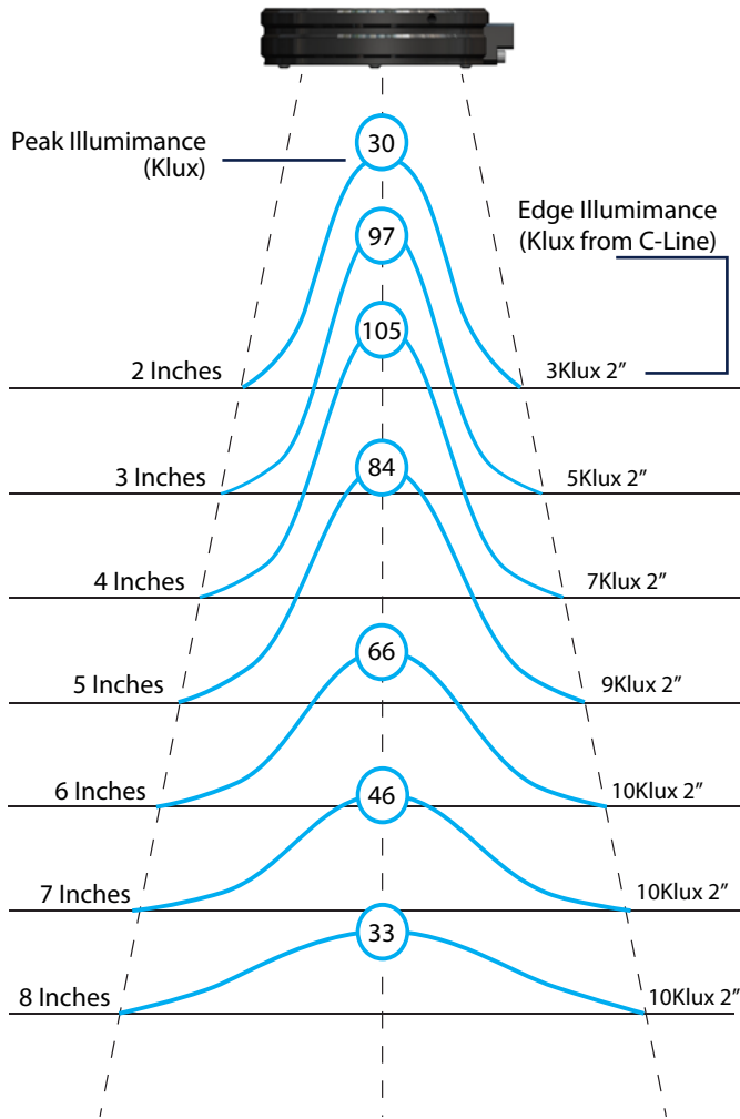
Illuminance Profiles at Various Working Distances
