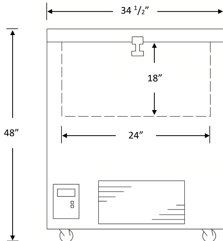
Chest Freezer Front View
