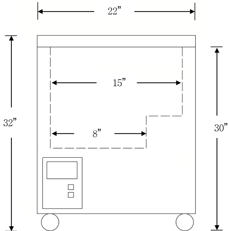
Chest Freezer Front View
