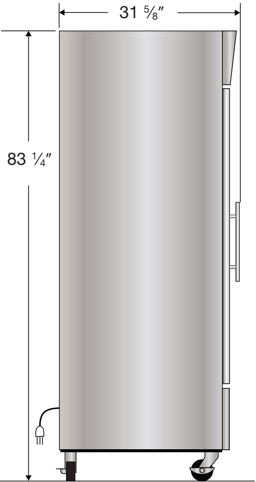
Side View
