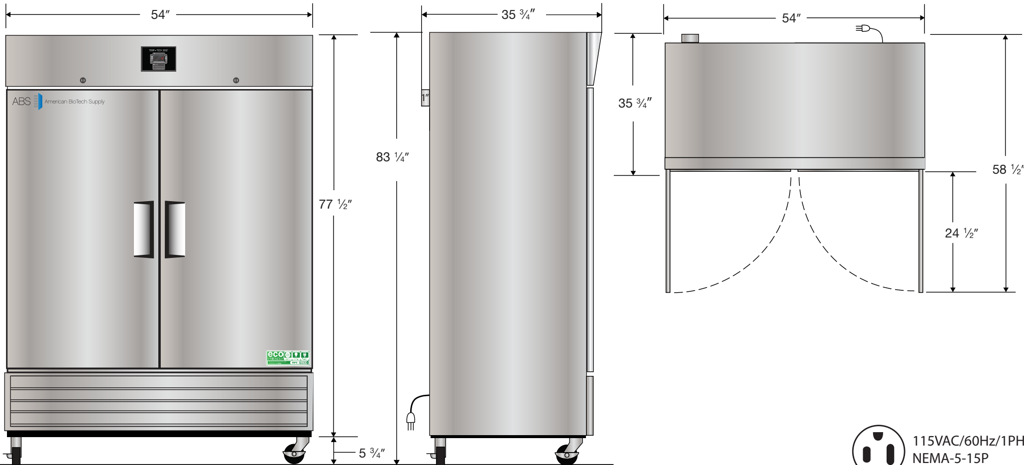
Top View
