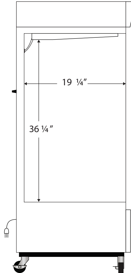
Side View
