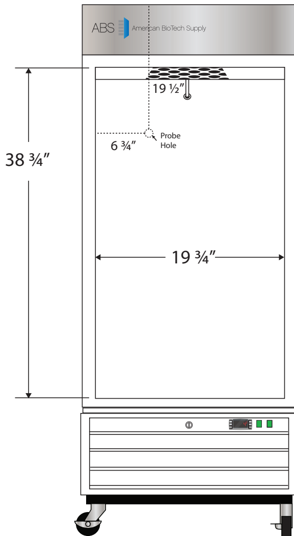
Front View
