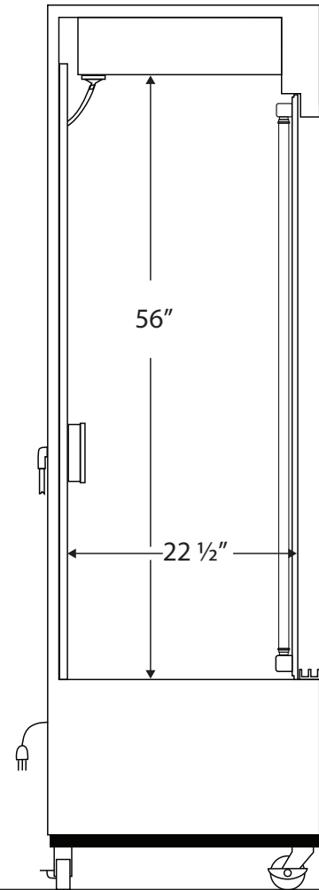
Side View
