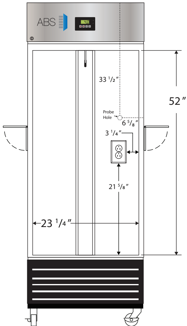
Front View
