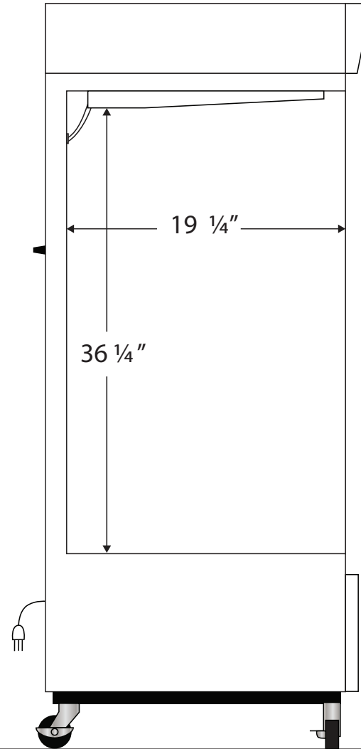
Side View
