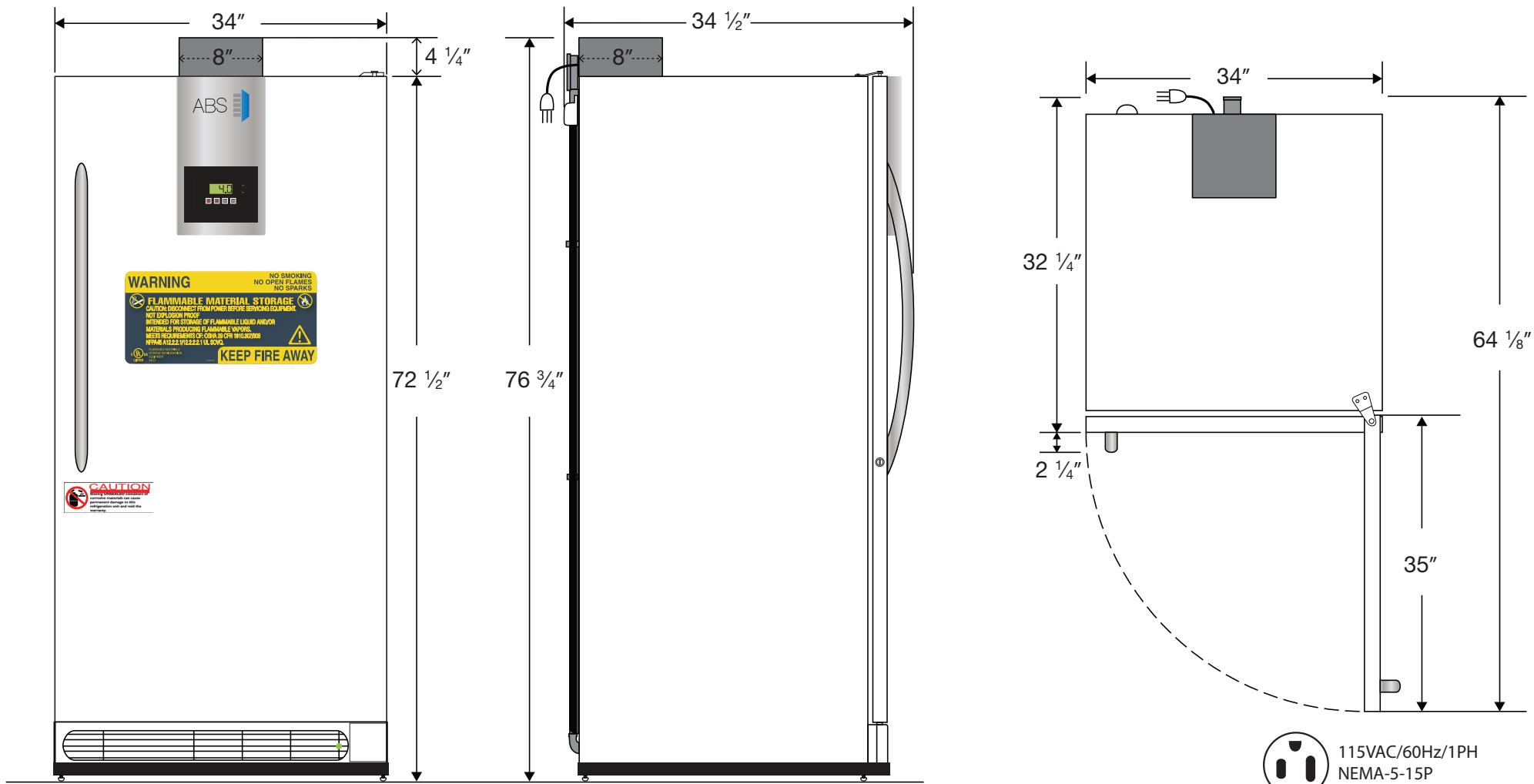
Top View
