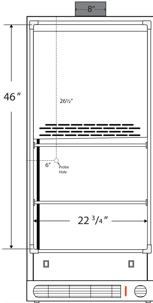
Front View
